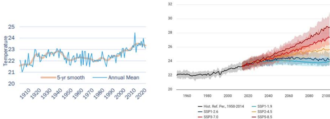
Figure 1: Observed Temperatures for Egypt [42]
